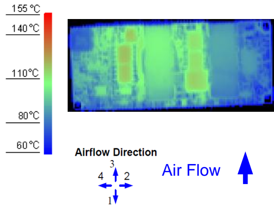
Figure 12. Thermal Image for Airflow Direction 3 (21.5A output, 55°C ambient, 200 LFM, V_{in} = 24V open frame unit)
