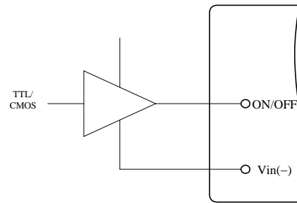
Figure 15. Direct Logic Drive
