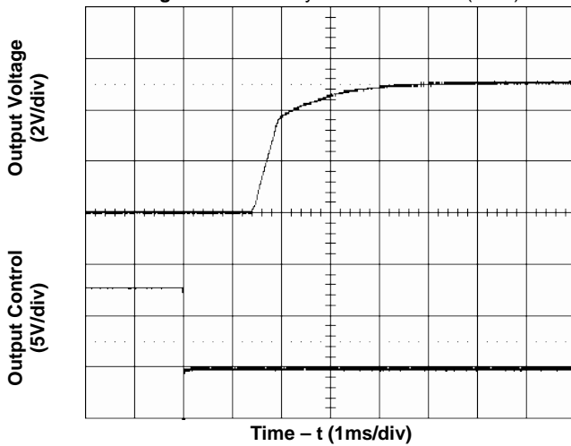
Figure 3. Start-Up from Enable Control (typical V_{in} and full load)
