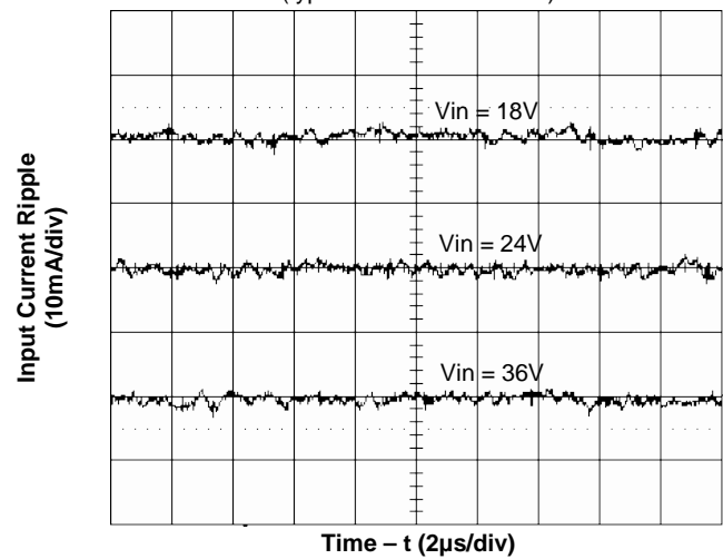
Figure 6. Input Reflected Ripple Current at Full Load
