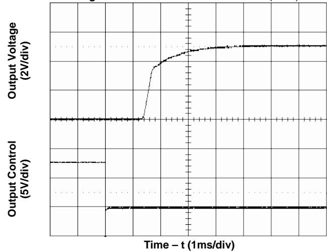
Figure 4. Start-Up from Enable Control (typical V_{in} and zero load)
