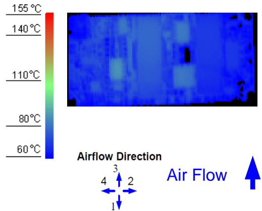
Figure 12. Thermal Image for Airflow Direction 3 (15A output, 55°C ambient, 200 LFM, V_{in} =24V open frame unit)
