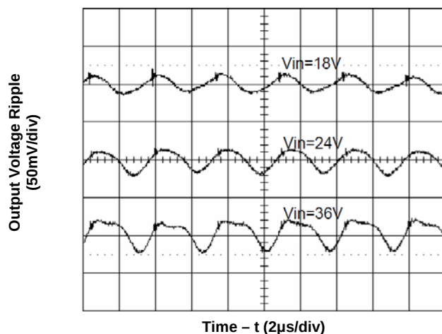
Figure 5. Output Ripple Voltage at Full Load
