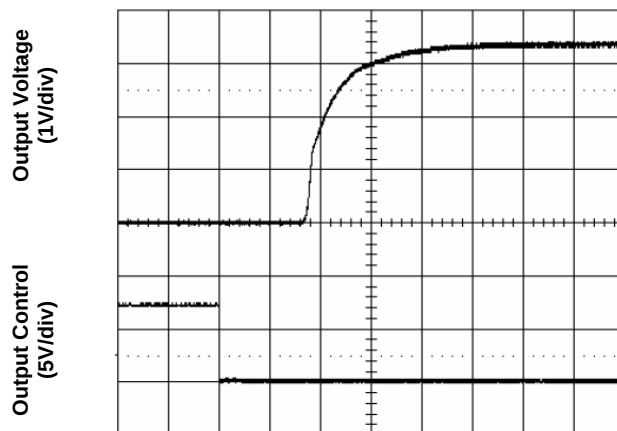
Figure 4. Start-Up from Enable Control (typical V_{in} and zero load)
