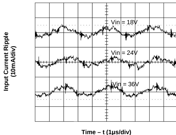
Figure 6. Input Reflected Ripple Current at Full Load
