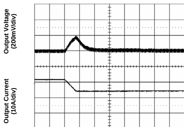
Figure 7. Transient Load Response
