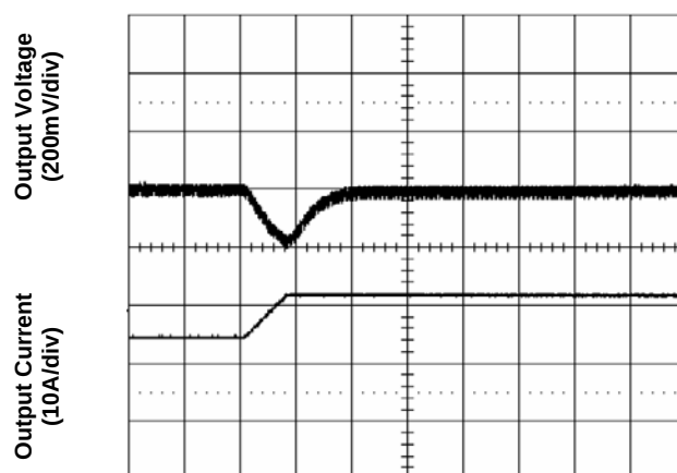
Figure 8. Transient Load Response
