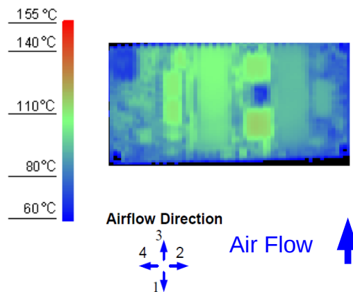
Figure 10. Thermal Image for Airflow Direction 3 (30A output, 55°C ambient, 200 LFM, V_{in} = 24V open frame unit)
