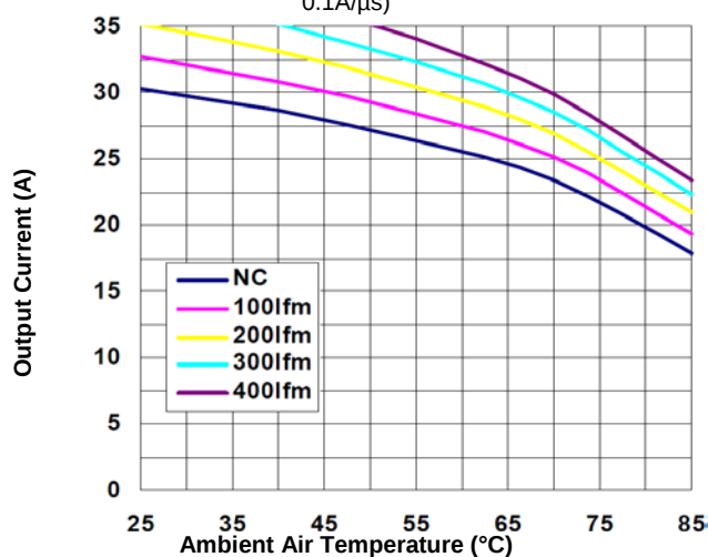
Figure 9. Current Derating Curve for Airflow Direction 3
