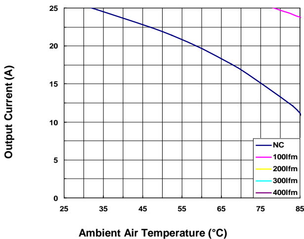
Figure 11. Current Derating Curve for Airflow Direction 3 (Ref. Fig. 12 for Airflow Direction; V_{in} = 24V, open frame unit using solder interface)
