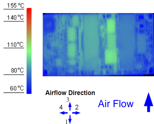
Figure 12. Thermal Image for Airflow Direction 3 (25A output, 55°C ambient, 200 LFM, V_{in} = 24V open frame unit)
