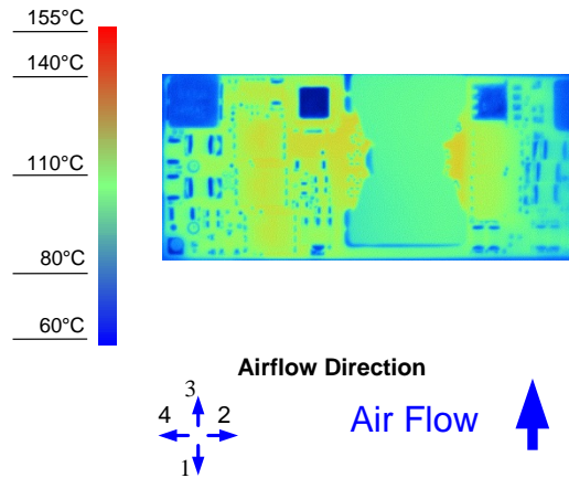
Figure 8. Thermal Image for Airflow Direction 3 (4.5A output, 55°C ambient, 200 LFM, typical Vin, open frame, unit soldered onto a fixture board)
