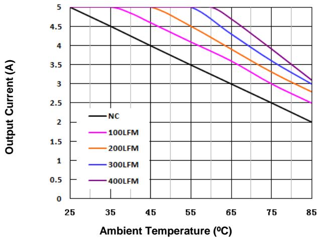
Figure 7. Current Derating Curve with Open Frame (Direction 3 (Ref. Figure 8); typical Vin, unit soldered onto a fixture board)
