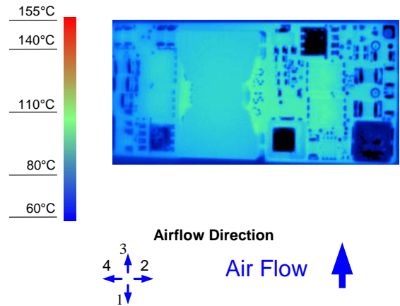
Figure 8. Thermal Image for Airflow Direction 3 (3A output, 55°C ambient, 200 LFM, typical Vin, open frame, unit soldered onto a fixture board)
