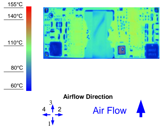
Figure 8. Thermal Image for Airflow Direction 3 (22A output, 55°C ambient, 200 LFM, typical Vin, open frame, unit soldered onto a fixture board)
