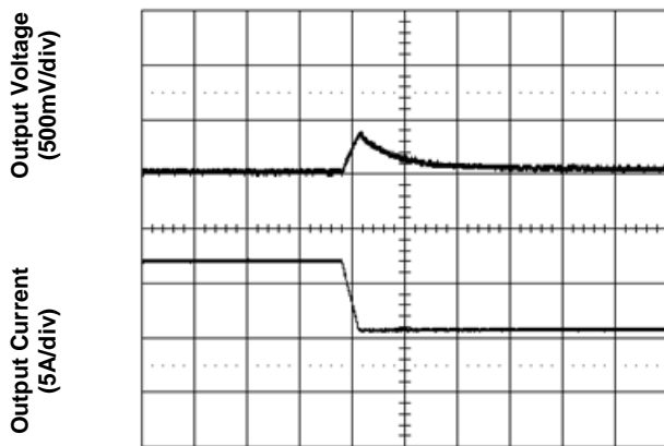
Figure 5. Transient Load Response (typical Vin, load current steps from 50% to 25% at a slew rate 0.1A/μs)
