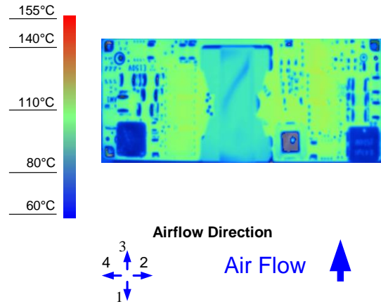
Figure 8. Thermal Image for Airflow Direction 3 (20A output, 55°C ambient, 200 LFM, typical Vin, open frame, unit soldered onto a fixture board)
