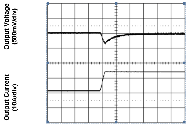
Figure 6. Transient Load Response (typical Vin, load current steps from 50% to 75% at a slew rate 0.1A/μs)
