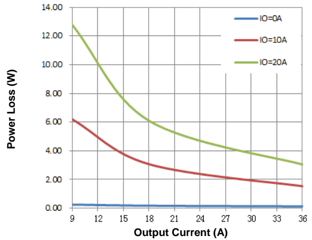
Figure 2. Power Loss vs. Load Current (25°C)
