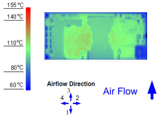
Figure 10. Thermal Image for Airflow Direction 3 (19A output, 55°C ambient, 200 LFM, typical Vin, open frame unit)
