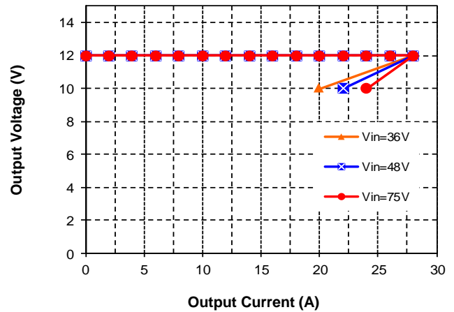
Figure 4. Output Characteristics (25°C)
