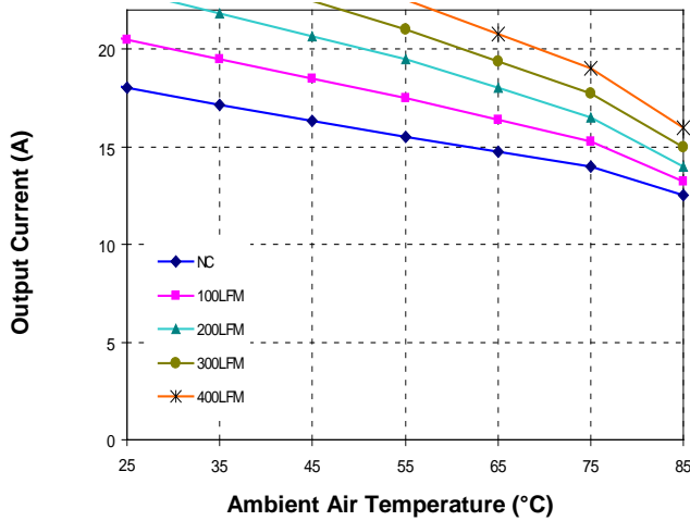
Figure 9. Current Derating Curve for Airflow Direction 3 (Ref. Fig. 10 for Airflow Direction; typical Vin, open frame)
