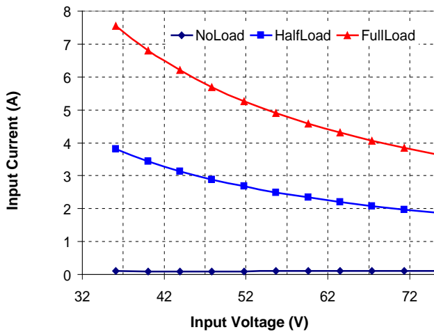
Figure 3. Input Characteristics (25°C)
