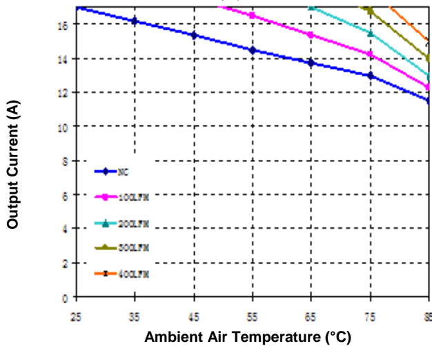
Figure 9. Current Derating Curve for Airflow Direction 3 (Ref. Fig. 10 for Airflow Direction; typical V_{in} , open frame)
