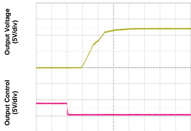
Figure 6. Start-Up from Enable Control (typical Vin, zero load, 1,000µF external output capacitance)
