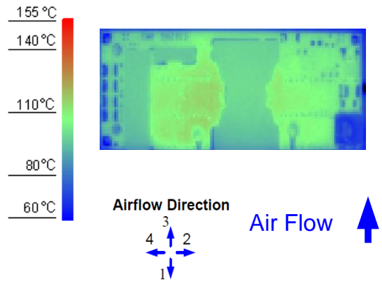
Figure 10. Thermal Image for Airflow Direction 3 (16.5A output, 55°C ambient, 100 LFM, typical V_{in} , open frame unit)
