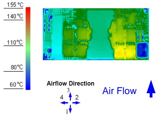
Figure 10. Thermal Image for Airflow Direction 3 (21A output, 55°C ambient, 200 LFM, typical Vin, open frame, unit soldered onto a fixture board)
