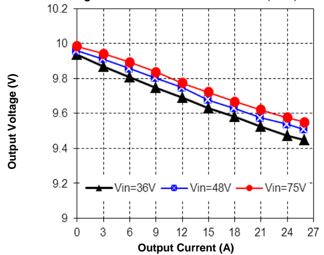
Figure 4. Output Characteristics (25°C) (Parallel version)
