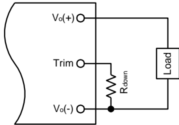
Figure 14. Circuit to Decrease Output Voltage
