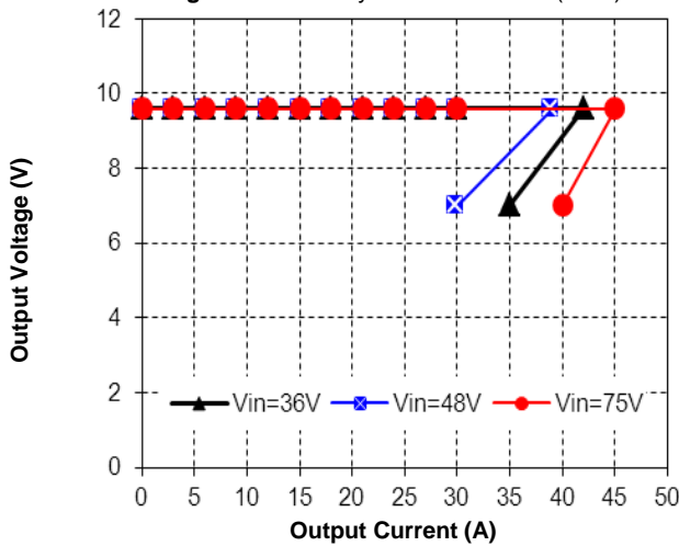
Figure 3. Output Characteristics (25°C) (Non-parallel version)
