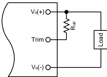
Figure 15. Circuit to Increase Output Voltage
