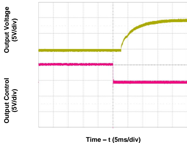
Figure 6. Start-Up from Enable Control (typical Vin, zero load, 1,000µF external output capacitance)
