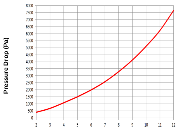
Coolant Flow (L/min.) Figure 1. Pressure Drop vs. Coolant Flow
